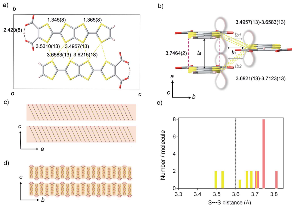
Fig. 2 Crystal structure of TED. (a) A unit cell projected on the a -axis, represented with black square, consisting of two TED molecules with intermolecular distances of S\cdots S contacts (yellow dotted line) and intramolecular hydrogen bond (black dotted line) in unit of Ångstrom. (b) A molecular stacking unit along the a and b -axes. Red break and yellow dotted lines show face-to-face and side-by-side intermolecular distances of S\cdots S contacts, where \pi -orbital orbitals overlap longitudinally along the a -axis and transversely along the b -axis, respectively, as is guided with the lobe image. Black arrows display the transfer integrals t_a (599 meV), t_b (60 meV), which is averaged [ t_b = (t_{b1} (69 \text{ meV}) + t_{b2} (51 \text{ meV}))/2 ]. (c and d) Super-structures of the TED molecular units crossing the c -axis; (c) stacking along the a direction; electric conduction occurs predominantly within the TED molecular layer, (d) stacking along the b direction. Red and yellow shadows show the anisotropic conduction pathways with t_a and t_b , respectively, in contrast, inter-layer conduction along the c -axis are much lower with t_c \sim 0 . (e) Distribution of S\cdots S distance in one molecule with an indication of van der Waals sum distance (black dotted line). Only one site was counted in the nearest neighbors with the same symmetry operation. Red and yellow bars show the contact along the a -axis and the b -axis, respectively.
