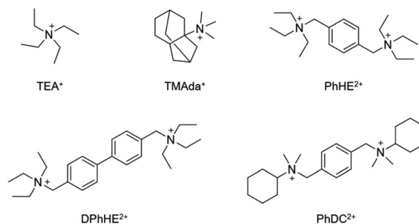
Scheme 1 Organic cations utilized as structure directing agents (OSDA).
