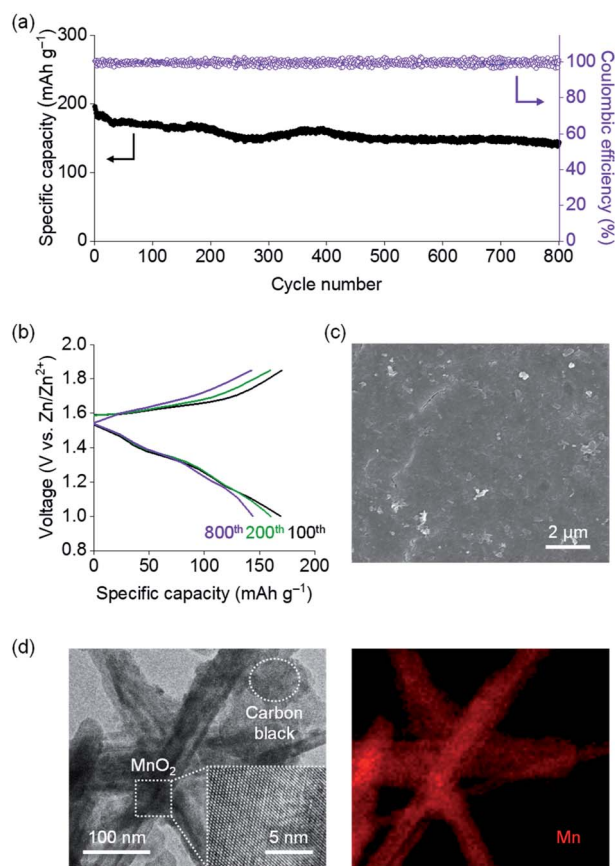
Fig. 4 (a) Cycling performance of a Zn|TpPa- \text{SO}_3\text{Zn}_{0.5} | \text{MnO}_2 cell. (b) Charge/discharge profiles at the 100 th , 200 th and 800 th cycles. (c) SEM image of the Zn metal anode after the 800 th cycle. (d) TEM (left) and EDS mapping (for Mn; right) images of the \text{MnO}_2 cathode after the 800 th cycle.
