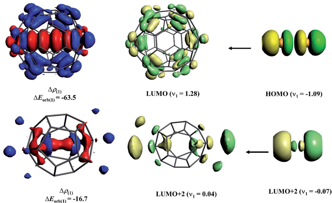
Fig. 7 Shape of the most important deformation density, \Delta\rho_{(1)} of \text{Xe}_2@\text{C}_{60} and \text{He}_2@\text{C}_{20}\text{H}_{20} corresponding to \Delta E_{\text{orb}(1)} in kcal mol ^{-1} and the associated fragment orbitals at the BP86-D3(BJ)-ZORA/TZ2P level. The eigenvalues \nu_n give the size of the charge migration in e. The direction of the charge flow of the deformation densities is red \rightarrow blue.
