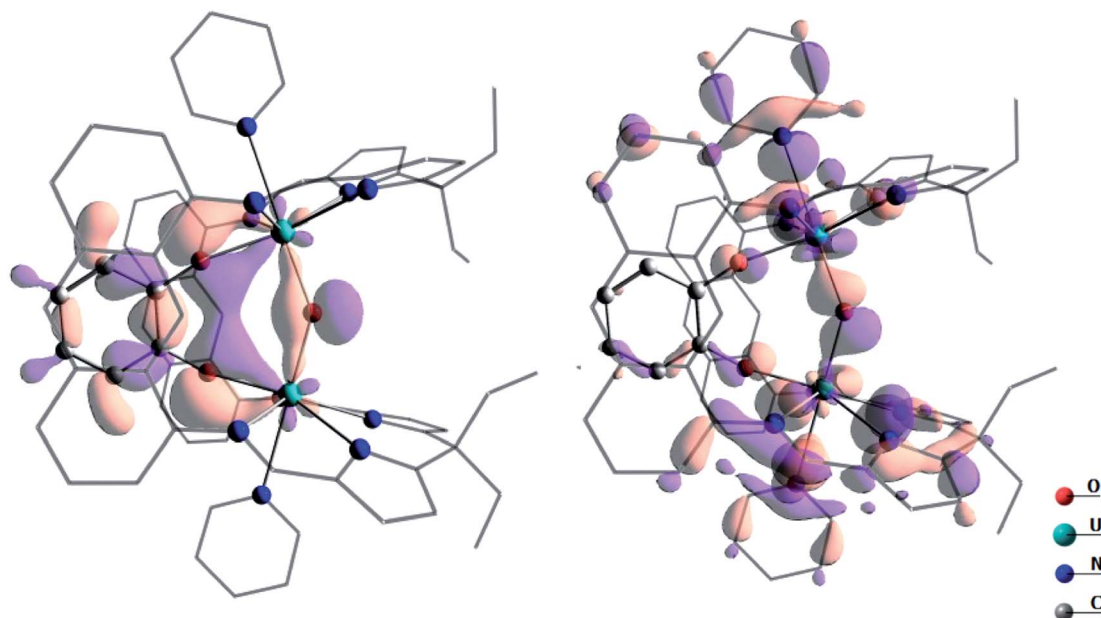
Fig. 7 Depiction of the two molecular orbitals describing the U–O bonding in complex A . These two orbitals are 2.42 eV lower in energy than the SOMO.
