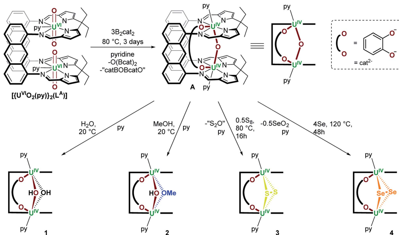
Scheme 1 Synthesis of [{(py)U^{IV}OU^{IV}(\mu-O_2C_6H_4)(py))}(L^A)] (A) from [{U^{VI}O_2(py)}_2(L^A)] and 3 equiv. of B_2cat_2 , 18 and subsequent synthesis of [{(py)U^{IV}(\mu-OH)_2U^{IV}(\mu-O_2C_6H_4)(py))}(L^A)] (1), [{(py)U^{IV}(\mu-OMe)(\mu-OH)U^{IV}(\mu-O_2C_6H_4)(py))}(L^A)] (2) and [{(py)U^{IV}(\mu-\eta^2-\eta^2-E)_2U^{IV}(\mu-O_2C_6H_4)(py))}(L^A)] ( E = S (3), Se (4)); py = pyridine.
