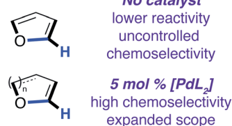
Fig. 1 C–O bond alumination of furans.
