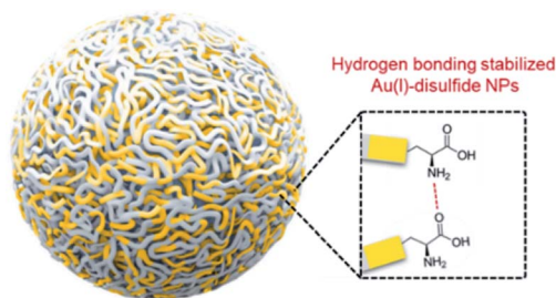
Scheme 2 Schematic illustration of the structure of Au(I)-disulfide NPs. The hydrogen bonds between Cys existed at the out layer of Au(I)-disulfide NPs, which maintain the structural stability of NPs in water.
