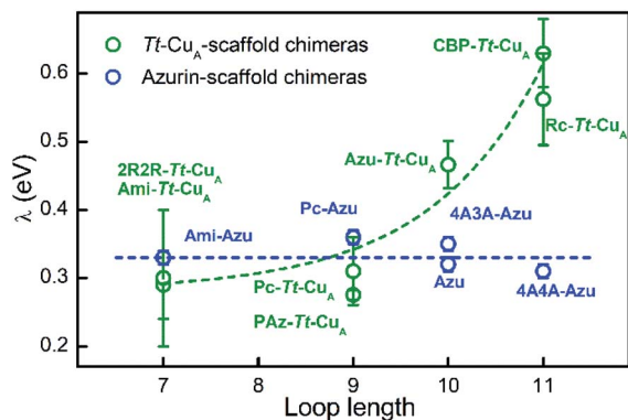
Fig. 6 Reorganization energies of Tt-Cu_A -based chimeras (green; this work) and azurin-based chimeras (blue; taken from Monari et al. 85 ) as a function of the length of the ligand loop. Dashed curves are included to guide the eye. Error bars represent the standard deviation of no less than 3 independent measures.
