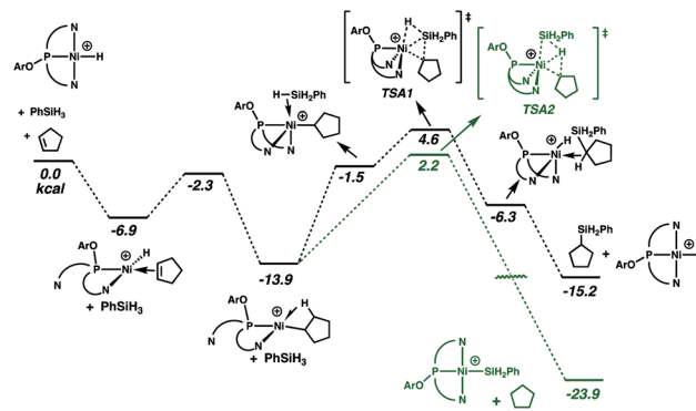
Fig. 2 Gibbs energy profile ( \text{kcal mol}^{-1} ) for cycle A of the hydrosilation catalyzed by [(\text{NPN})\text{NiH}]^+ .
