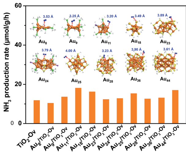
Fig. 1 The photocatalytic activity of the ligand-protected Au_n clusters supported on TiO_2-Ov for N_2 reduction. The inset shows the atomic structures of the Au_n clusters, which can only physisorb N_2 molecule with distance between N_2 and Au sites larger than 3.2 Å. The C, N, S, Au, P and Cl are shown in gray, blue, yellow, orange, green and violet colors, respectively. H atoms are omitted for clarity.
