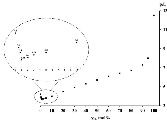
Fig. 1 \text{p}K_{\text{a}} values of \text{PhCH}(\text{CN})_2 versus the molar fractions \chi_{\text{IL}} of [Bmim][NTf 2 ] in [Bmim][NTf 2 ]/DMSO mixtures.
