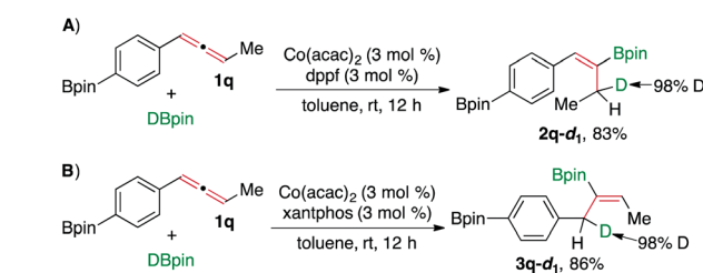
Scheme 3 Deuterium-labelling experiments.
