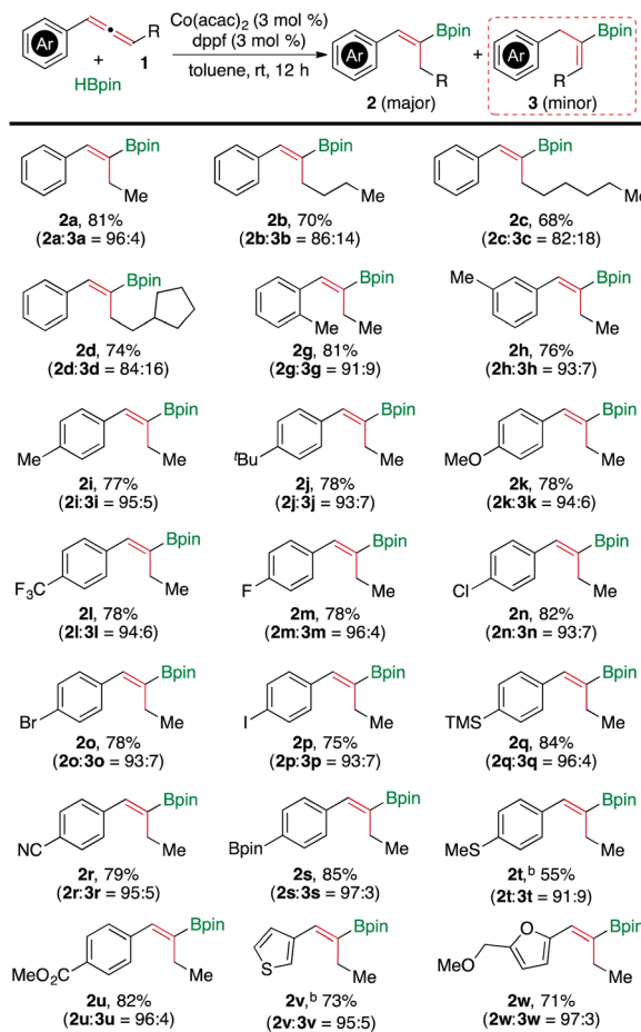
Fig. 2 \text{Co}(\text{acac})_2/\text{dppf} -catalyzed hydroboration of internal allenes. a Conditions: allene (0.400 mmol), HBpin (0.440 mmol), \text{Co}(\text{acac})_2 (12 \mu\text{mol} ), dppf (12 \mu\text{mol} ), toluene (1 mL), room temperature, 12 h, and isolated yields after column chromatography; b 18 h.
