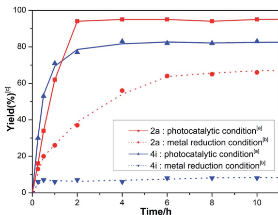
Fig. 3 Reaction profiles for 2a and 4i (200 mg, 0.1 M in THF). [a] Photocatalytic conditions: 450 nm 10 W LED, 1a (1 mol%), \text{Cp}_2\text{TiCl}_2 (5 mol%), HE (1.2 eq.). [b] Metal reduction conditions: \text{CpTi}_2\text{Cl}_2 (5 mol%), Zn (2.0 eq.), coll·HCl (2.5 eq.). [c] The yields of 3a or 5i were determined with ^1\text{H} NMR.
