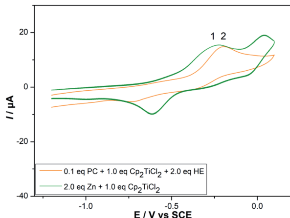
Fig. 2 Cyclic voltammetry of 2 mM \text{Cp}_2\text{TiCl}_2/\text{Zn} (green line) and 2 mM \text{Cp}_2\text{TiCl}_2/\text{Ir}(\text{dtbbpy})(\text{ppy})_2\text{PF}_6/\text{HE} (orange line) recorded on a glassy carbon disk electrode with \nu = 0.1 \text{ V s}^{-1} in 0.2 M \text{Bu}_4\text{NPF}_6/\text{THF} . Experimental details are found in the ESI, S4.† The values are given in V vs. SCE and can be converted to V vs. \text{Fc}^+/\text{Fc} by subtracting 0.52 V.
