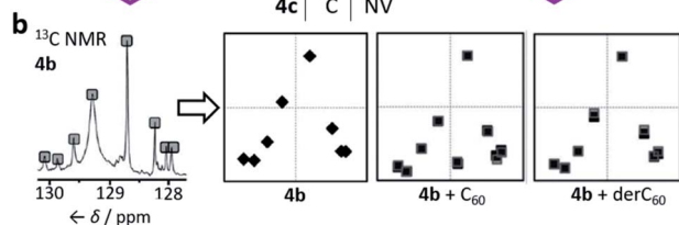
Fig. 4 (a) Bode's bisporphyrin-bullvalene 4 , which was prepared with natural isotopic abundance ( 4a ), enriched in ^{13}\text{C} at one position ( 4b ) of the dynamic C 10 core, and functionalised with a photocleavable group ( 4c ). (b) The complex ^{13}\text{C} NMR spectra of the dynamic mixtures are converted to simplified representations, showing that the ^{13}\text{C} NMR spectrum of a 4b mixture at equilibrium changes in the presence of fullerene guests. NMR data (150 MHz, solutions in CS 2 with 3% CD 2 Cl 2 ) shown for samples of: ( 4b ) 2.8 mM 4b ; ( 4b + C 60 ) 2.8 mM 4b with 2 equiv. C 60 ; ( 4b + derC 60 ) 2.8 mM 4b with 4 equiv. derC 60 . The representations of NMR spectra correspond to two trials overlaid. NV = o -nitroveratryl. Adapted from ref. 7e with permission from The Royal Society of Chemistry.
