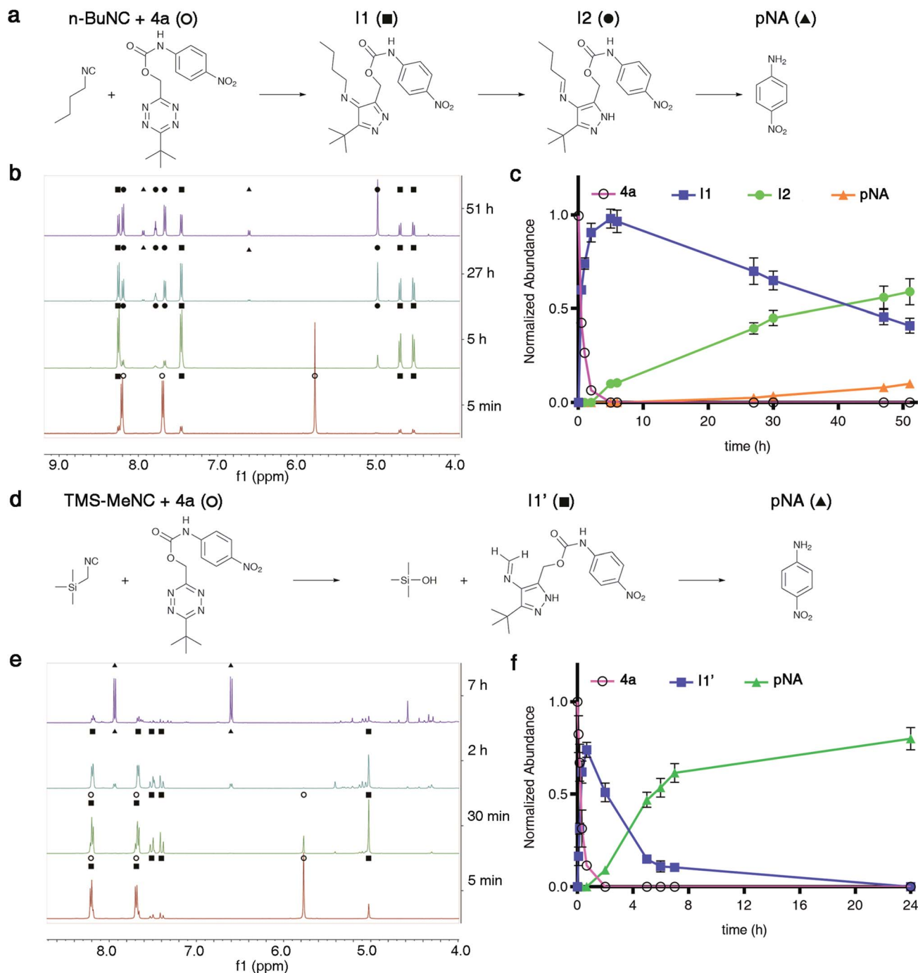
Fig. 4 1 H-NMR analysis of reactions between isocyanides n -BuNC or TMS-MeNC and 4a to liberate pNA. (a and d) Proposed intermediates in the reaction between n -BuNC (a) or TMS-MeNC (d) and 4a leading to the release of pNA. (b and e) Time-dependent 1 H-NMR of the reaction progress between n -BuNC (b) or TMS-MeNC (e) and 4a ( c (4a) = 6 mM, c (R-NC) = 15 mM, DMSO- d 6 : D 2 O (9 : 1, v/v), T = 25 °C, expanded spectra in ESI). (c and f) Normalized amount of starting material (4a), subsequent intermediates, and pNA formed as a function of time.
