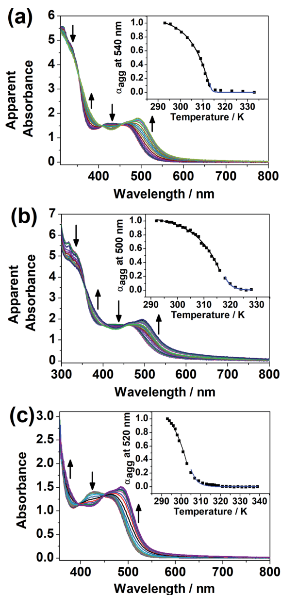
Fig. 4 UV-Vis absorption spectra of (a) 1 ([Pt] = 2.8 \times 10^{-4} M), (b) 3 ([Pt] = 2.8 \times 10^{-4} M) and (c) 4 ([Pt] = 1.6 \times 10^{-4} M) in DMSO upon decreasing temperature (a) from 333 to 293 K, (b) from 328 to 292 K and (c) from 339 to 293 K. The apparent absorbance values were obtained by correcting to a 1 cm path length equivalence. Insets: plots of degree of aggregation against temperature for the cooling of the DMSO solutions of the complexes. The solid lines show the fitted curves in the elongation (black) and the nucleation (blue) regimes.
