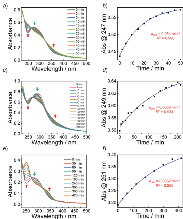
Fig. 4 (a, c and e) Absorbance spectra and (b, d and f) absorbance intensity changes together with a mono-exponential fit of aqueous dispersions ( 0.1 \text{ g L}^{-1} , 25^\circ \text{C} ) of (a and b) BP1 vesicles, (c and d) BP2 vesicles, and (e and f) BP3 micelles under UV 365 nm irradiation ( 4 \text{ mW cm}^{-2} ).
