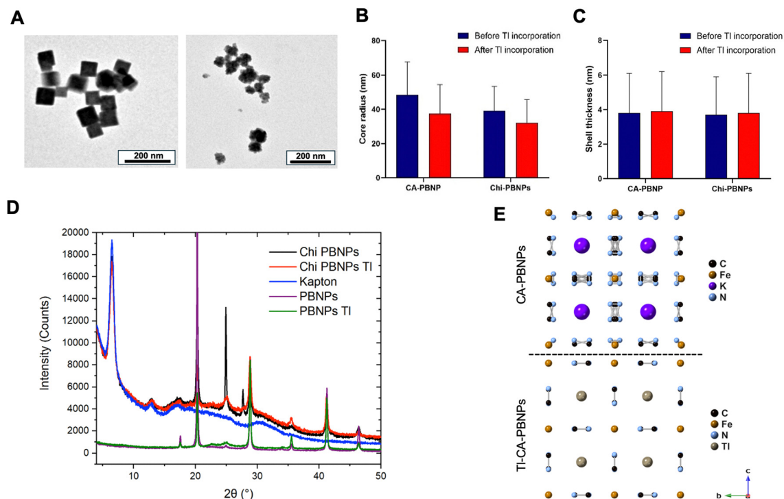
Fig. 4 (A) Transmission electron microscopy (TEM) images of \text{Tl}^+ -doped Prussian blue nanoparticles coated with citric acid (Tl-CA-PBNPs, left) and with chitosan (Tl-Chi-PBNPs, right) (see Fig. 2A for comparison with Tl-free particles). TEM images revealed no significant changes in shape or size compared to the non-doped samples; (B) average core radius (nm) obtained from the small-angle X-ray scattering (SAXS) fitting data for CA-PBNPs, Chi-PBNPs, Tl-CA-PBNPs and Tl-Chi-PBNPs; (C) Average shell thickness (nm) obtained from the small-angle X-ray scattering (SAXS) fitting data for CA-PBNPs, Chi-PBNPs, Tl-CA-PBNPs and Tl-Chi-PBNPs. SAXS measurements showed that core radius and shell thickness for both of PBNPs was not affected by Tl incorporation; (D) X-ray diffraction (XRD) spectra for CA-PBNPs, Chi-PBNPs, Tl-CA-PBNPs and Tl-Chi-PBNPs. XRD results showed a large impact of thallium loading on the diffraction intensities for both samples; (E) schematic representation of the crystal structure for CA-PBNPs (top) and Tl-CA-PBNPs (bottom) obtained by Rietveld refinement of the XRD data which confirmed that \text{Tl}^+ is located in interstitial spaces within the crystal structure of the nanoparticles. For CA-PBNPs the refinements were obtained on the assumption that the interstitial spaces are occupied (e.g., by potassium).
