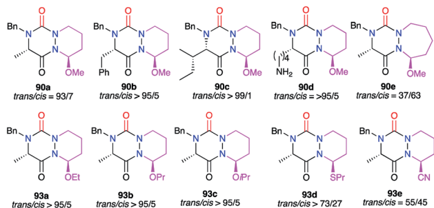
Scheme 34 One-pot synthesis of bicyclic functionalised aza-DKPs.
