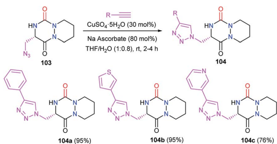
Scheme 38 Triazole formation at position 5 via Cu-catalysed [3 + 2] cycloaddition.
