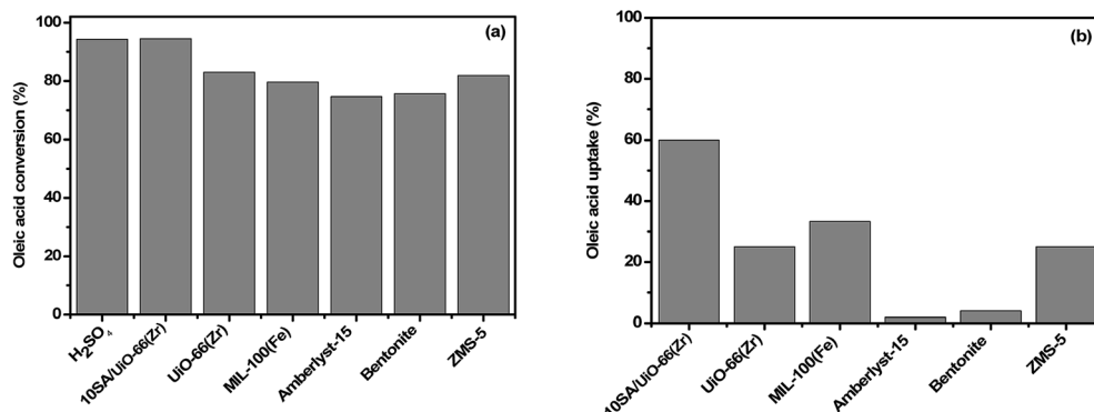
Fig. 12 Comparison of the (a) catalytic activities and (b) adsorption capabilities of 10SA/UiO-66(Zr) and other reported catalysts for oleic acid.
