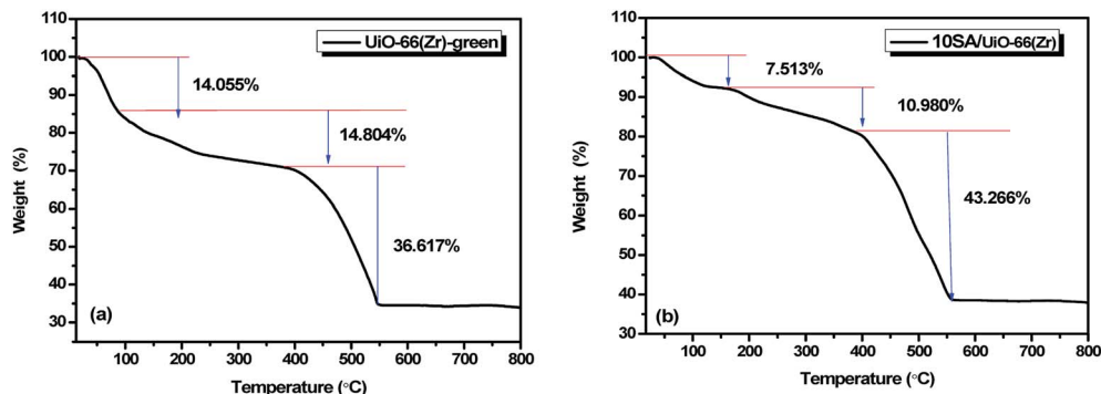
Fig. 7 TGA curves of (a) UiO-66(Zr)-green and (b) 10SA/UiO-66(Zr).
