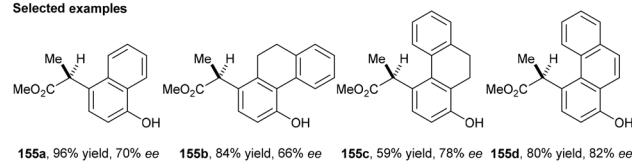
Scheme 45 NHC-catalyzed intramolecular benzannulation to synthesize multi-functionalized phenols.
