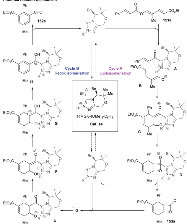
Scheme 44 NHC-catalyzed intramolecular benzannulation to synthesize tri-substituted benzaldehydes.
