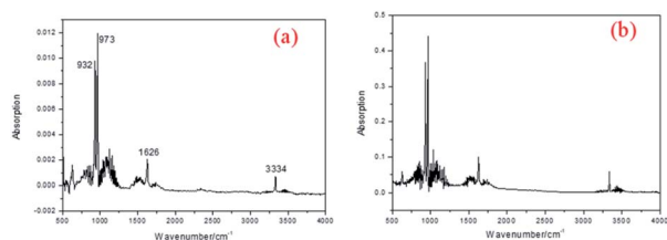
Fig. 7 The IR spectrum when connecting pipe temperature is 50 °C (a) and standard IR spectrum of \text{NH}_3 (b).
