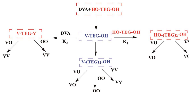
Fig. 8 Scheme of reaction sequences in the transesterification of DVA with TEG. 115
