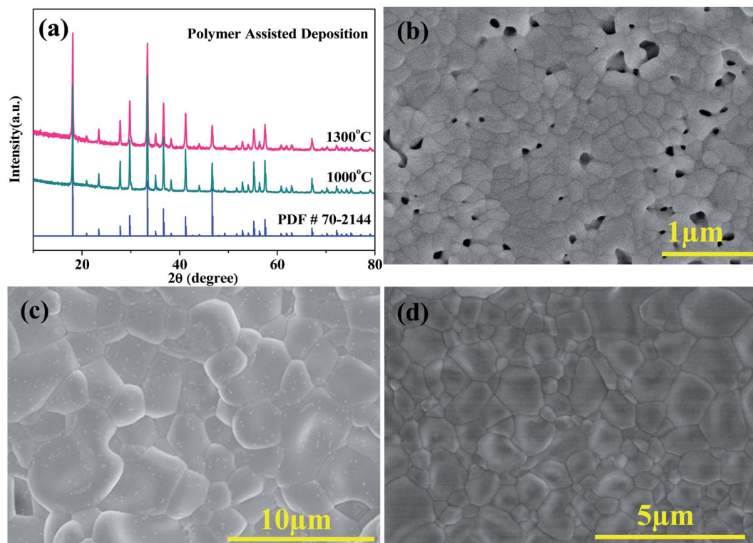
Fig. 1 (a) XRD patterns of the \text{Ca}_{12}\text{Al}_{14}\text{O}_{33} samples from PAD method calcined at 1000 °C and 1300 °C, (b) and (c) show the microstructures of samples firing at 1000 °C and 1300 °C, respectively; (d) presents the particle size of the ceramic sample prepared by SSR method at 1300 °C.
