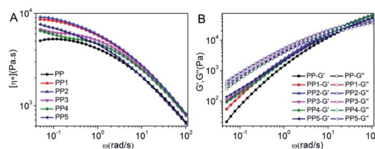
Fig. 2 Polypropylene matrix composite [\eta^*]-\omega curves (A), and G' and G''-\omega curves (B), with the low-frequency energy storage modulus ( G' ) and low-frequency.
