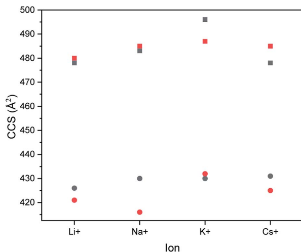
Fig. 3 Calculated CCS of the hexamers with different adducts. Singly charged states (black symbols) and doubly charged states (red symbols) are shown for the B 3 T 3 structures (squares) and (BT) 3 structures (dots).
