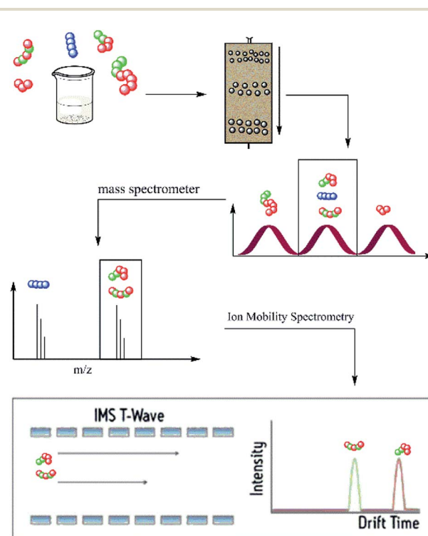
Scheme 1 Scheme of oligomer separation in APC-MS-IMS measurements.
