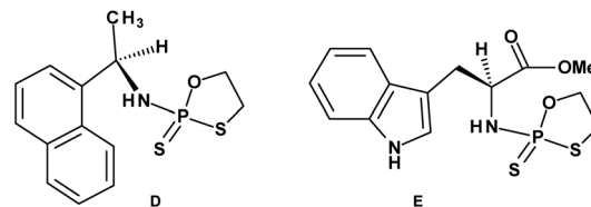
Chart 2 (D) (R_c) -2-(1-( \alpha -Naphthyl)ethyl)amino)-2-thio-1,3,2-oxathiaphospholane, (E) a 2-thio-1,3,2-oxathiaphospholane derivative of L-tryptophan methyl ester; N_{NPS}N' -Trp.
