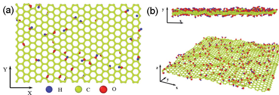
Fig. 1 The simulation model of GO based on the Lorf–Klinowski model, (a) the original atomic structure of GO, (b) the cross and side view of relaxed atomic structure of GO at 300 K for 2.5 ns, the average interlayer distances are 3.4 Å, carbon, oxygen, and hydrogen atoms are represented by yellow, red, and blue, respectively.
