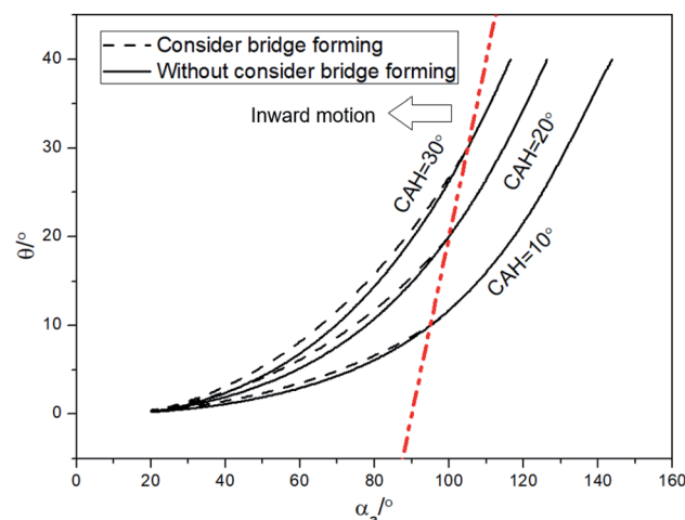
Fig. 9 Comparisons of results between considering and without considering bridge forming by theoretical analysis.
