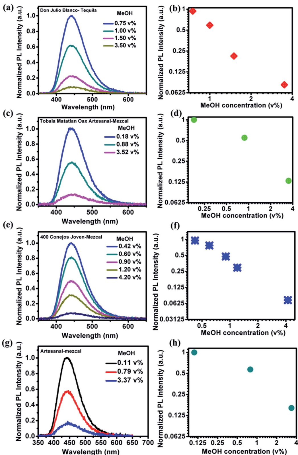
Fig. 6 Fluorescence response of NOCDs (measured at \lambda_{\text{ex}} = 340 \text{ nm} ) in the presence of some tested spiked branded and unbranded alcoholic beverages after dilution (a and b) Don Julio Blanco-Tequila (tDJB), (c and d) Tobala Matatlan Oax Artesanal (traditional branded)-Mezcal (mTMOA), (e and f) 400 Conejos Joven-Mezcal (m400CJ) and (g and h) (traditional unbranded) Artesanal mezcal (mAR).
