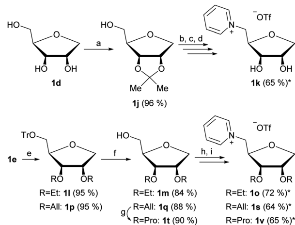
Fig. 3 Synthesis of alternative 1-deoxy-ribose ILs with varying 2- and 3- O -groups. (a) 2,2-Dimethoxy propane, camphorsulfonic acid, acetone, r.t., 1.5 h; (b) \text{Tf}_2\text{O} , pyridine, DCM, 0^\circ\text{C} , 10 min; (c) pyridine, reaction at rotary evaporator, 700 mbar, 40^\circ\text{C} ; (d) AcOH (70%), r.t., 20 min; (e) NaH, ethyl or allyl bromide, DMF, 0^\circ\text{C} \geq \text{r.t.} , overnight; (f) AcOH (70%), 70^\circ\text{C} , 45 min; (g) \text{Pd}(\text{OH})_2 , MeOH, \text{H}_2 -atmosphere, r.t., 12 h; (h) \text{Tf}_2\text{O} , pyridine, DCM, 0^\circ\text{C} , 10 min; (i) pyridine, reaction at rotary evaporator, 700 mbar, 40^\circ\text{C} ; *yield over two steps.
