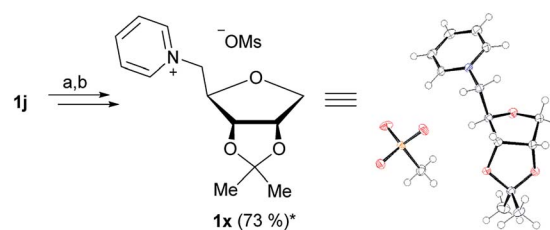
Fig. 4 Synthesis and ORTEP 13 of 1x . (a) Mesyl chloride, pyridine, r.t., 12 h; (b) pyridine, 125^\circ\text{C} , 5 h; *yield over two steps.
