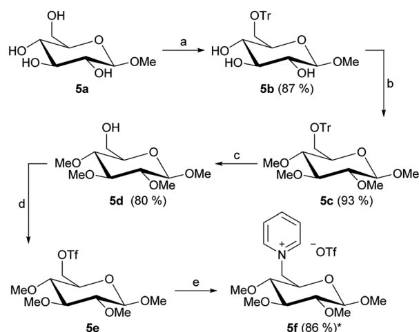
Fig. 6 Synthesis of ionic liquid 5f from \beta -D-methyl glucoside 5a; the same strategy was applied for \beta -allyl glucoside (6a–f), \beta -phenyl glucoside (7a–f) and \alpha -methyl glucoside (8a–f). (a) Trityl chloride, \text{NEt}_3 , DMAP, DCM, r.t., overnight; (b) NaH, MeI, DMF, 0^\circ\text{C} \geq \text{r.t.} , overnight; (c) AcOH (70%), 70^\circ\text{C} , 45 min; (d) \text{Tf}_2\text{O} , pyridine, DCM, 0^\circ\text{C} , 10 min; (e) pyridine, reaction at rotary evaporator, 700 mbar, 40^\circ\text{C} ; *yield over two steps.
