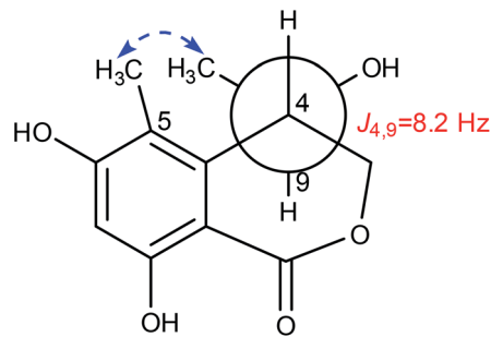
Fig. 7 The key NOESY correlation of 3 .
