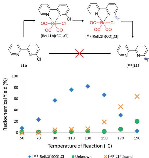
Fig. 3 [\text{F}^{18}]\text{Fluoride} substitution in the ortho position of [\text{Re}(\text{L1b})(\text{CO})_3\text{Cl}] which afforded [\text{F}^{18}]\text{Re}(\text{L1f})(\text{CO})_3\text{Cl} (blue diamonds). Thermal decomplexation led to the subsequent formation of [\text{F}^{18}]\text{L1f} (orange crosses) and an unknown by-product (green circles) with the RCYs plotted as a function of reaction temperature. [\text{F}^{18}]\text{L1f} was unable to be synthesised from L1b without first complexing to a rhenium(i) centre.
