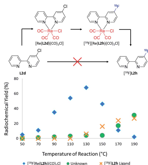
Fig. 4 RCYs of [\text{F}^{18}][\text{Re}(\text{L2h})(\text{CO})_3\text{Cl}] (blue diamonds), [\text{F}^{18}]\text{L2h} (orange crosses) and an unknown by-product (green circles) plotted as a function of the reaction temperature for the [\text{F}^{18}]\text{fluoride} labelling of the para substituted [\text{Re}(\text{CO})_3(\text{L2d})\text{Cl}] complex. [\text{F}^{18}]\text{L2h} was unable to be synthesised from L2d unless mediated by rhenium(i) complexation as per the above scheme.
