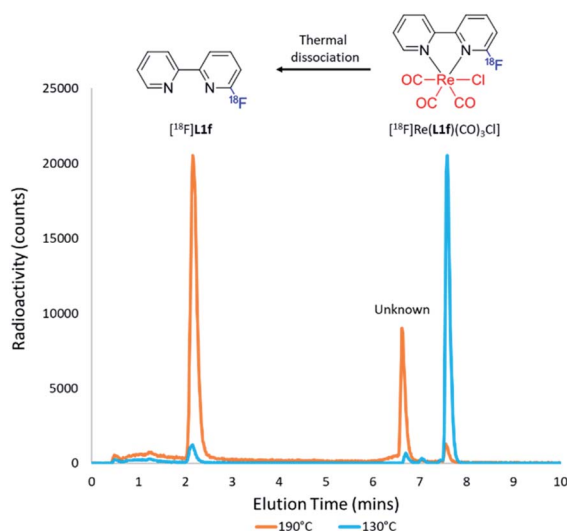
Fig. 2 Radiochromatogram profiles for the fluorine-18 labelling of [\text{Re}(\text{L1b})(\text{CO})_3\text{Cl}] at 130 °C (blue trace) and 190 °C (orange trace). At 130 °C [\text{F}^{18}]\text{Re}(\text{L1f})(\text{CO})_3\text{Cl} (7.6 min) forms in the greatest yield, whereas at 190 °C the complex dissociates to form the otherwise unobtainable [\text{F}^{18}]\text{L1f} ligand (2.2 min) alongside an unknown by-product (6.6 min).
