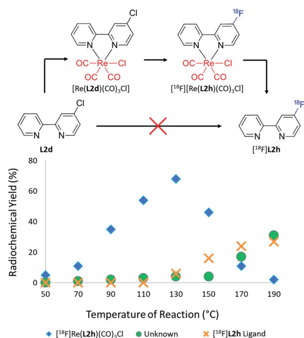
Fig. 4 RCYs of ^{18}\text{F}[\text{Re}(\text{L2h})(\text{CO})_3\text{Cl}] (blue diamonds), ^{18}\text{F}[\text{L2h}] (orange crosses) and an unknown by-product (green circles) plotted as a function of the reaction temperature for the ^{18}\text{F} fluoride labelling of the para substituted [\text{Re}(\text{CO})_3(\text{L2d})\text{Cl}] complex. ^{18}\text{F}[\text{L2h}] was unable to be synthesised from L2d unless mediated by rhenium(i) complexation as per the above scheme.
