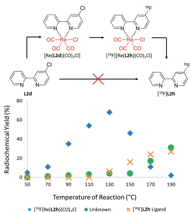
Fig. 4 RCYs of [\text{18F}][\text{Re}(\text{L2h})(\text{CO})_3\text{Cl}] (blue diamonds), [\text{18F}]\text{L2h} (orange crosses) and an unknown by-product (green circles) plotted as a function of the reaction temperature for the [\text{18F}] fluoride labelling of the para substituted [\text{Re}(\text{CO})_3(\text{L2d})\text{Cl}] complex. [\text{18F}]\text{L2h} was unable to be synthesised from \text{L2d} unless mediated by rhenium(i) complexation as per the above scheme.
