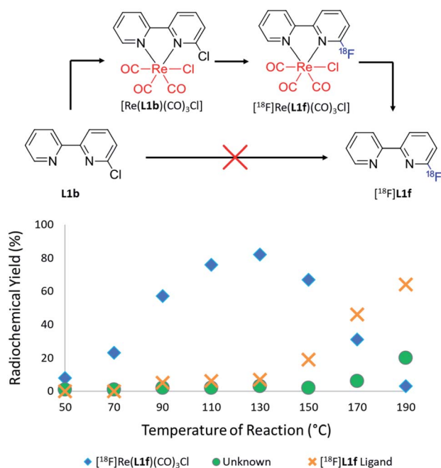
Fig. 3 [\text{18F}] Fluoride substitution in the ortho position of [\text{Re}(\text{L1b})(\text{CO})_3\text{Cl}] which afforded [\text{18F}][\text{Re}(\text{L1f})(\text{CO})_3\text{Cl}] (blue diamonds). Thermal decomplexation led to the subsequent formation of [\text{18F}]\text{L1f} (orange crosses) and an unknown by-product (green circles) with the RCYs plotted as a function of reaction temperature. [\text{18F}]\text{L1f} was unable to be synthesised from \text{L1b} without first complexing to a rhenium(i) centre.
