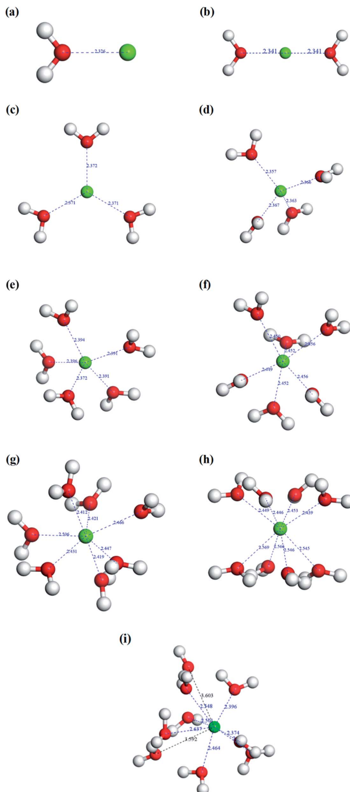
Fig. 5 Coordination simulation of hydrated calcium ions with different water molecules. (a) \text{Ca}[\text{H}_2\text{O}]^{2+} , (b) \text{Ca}[\text{H}_2\text{O}]_2^{2+} , (c) \text{Ca}[\text{H}_2\text{O}]_3^{2+} , (d) \text{Ca}[\text{H}_2\text{O}]_4^{2+} , (e) \text{Ca}[\text{H}_2\text{O}]_5^{2+} , (f) \text{Ca}[\text{H}_2\text{O}]_6^{2+} , (g) \text{Ca}[\text{H}_2\text{O}]_7^{2+} , (h) \text{Ca}[\text{H}_2\text{O}]_8^{2+} , and (i) \text{Ca}[\text{H}_2\text{O}]_9^{2+} .
