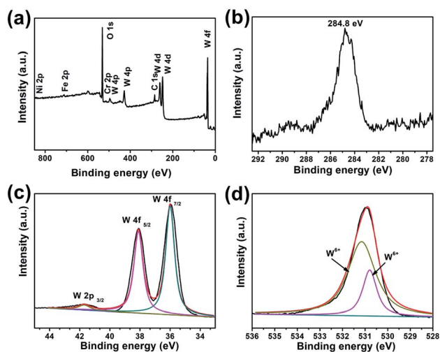
Fig. 3 XPS spectra of furball-like \text{WO}_3 microspheres sample: (a) survey XPS spectrum, (b) core-level XPS spectra of (b) C 1s, (c) W 4f, and (d) O 1s.
