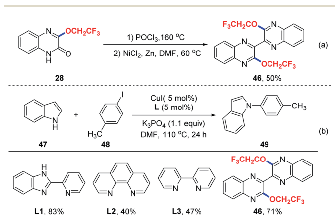
Scheme 3 Further chemistry.
