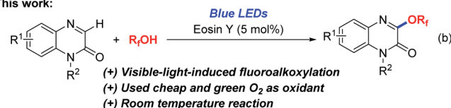
Scheme 1 The C3–H fluoroalkoxylation of quinoxalin-2(1 H )-ones.
