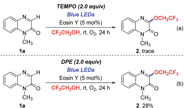
Scheme 4 Mechanism studies.
