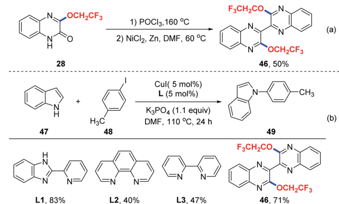
Scheme 3 Further chemistry.
