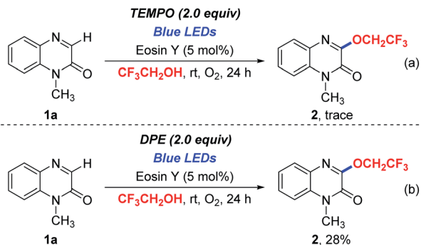
Scheme 4 Mechanism studies.
