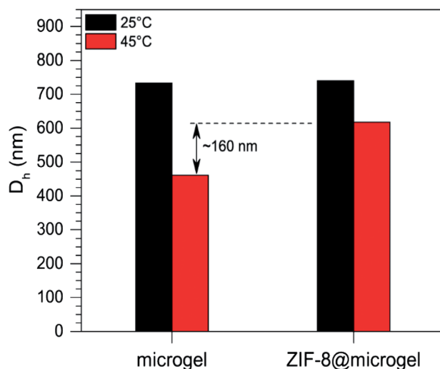
Fig. 6 Size transition comparison for microgel and ZIF-8@microgel particles between 25 °C and 45 °C as measured from DLS experiments.
