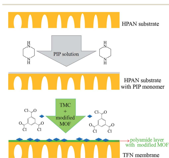
Fig. 1 Schematic diagram of the preparation process of TFN membranes.
