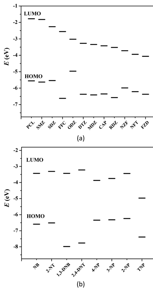
Fig. 4 HOMO and LUMO energy levels for the selected antibiotics (a) and nitroaromatics explosives (b).
