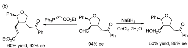
Scheme 21 Oxa-Michael cascade reaction for the synthesis of chiral tetrahydrofuran derivatives and the derivatization of chiral tetrahydrofuran.
