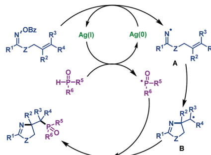
Scheme 20 Proposed mechanism.
