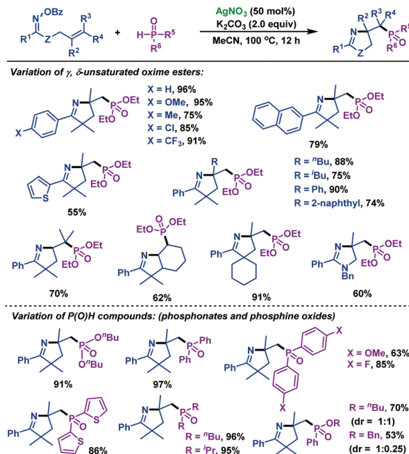
Scheme 19 Zhu and Chen's silver-promoted imino-phosphorylation of \gamma,\delta -unsaturated oxime esters with P(\text{O})\text{H} compounds.
