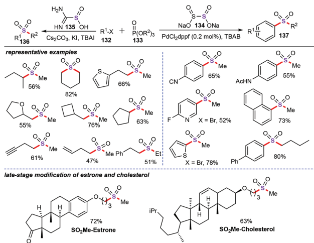
Scheme 50 General sulfone construction via \text{SO}_2 surrogate control.
