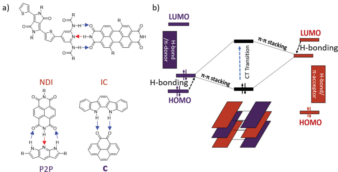
Scheme 1 (a) Previously reported H-bonded multicomponent semiconductors 22,39,40 (blue arrows show proton displacement from electron donor to acceptor and red arrows show proton displacement from electron acceptor to donor), (b) Energy diagram of donor (left), acceptor (right), and CT state (middle). Black arrows show change in the HOMO/LUMO energy level upon H-bonding.
