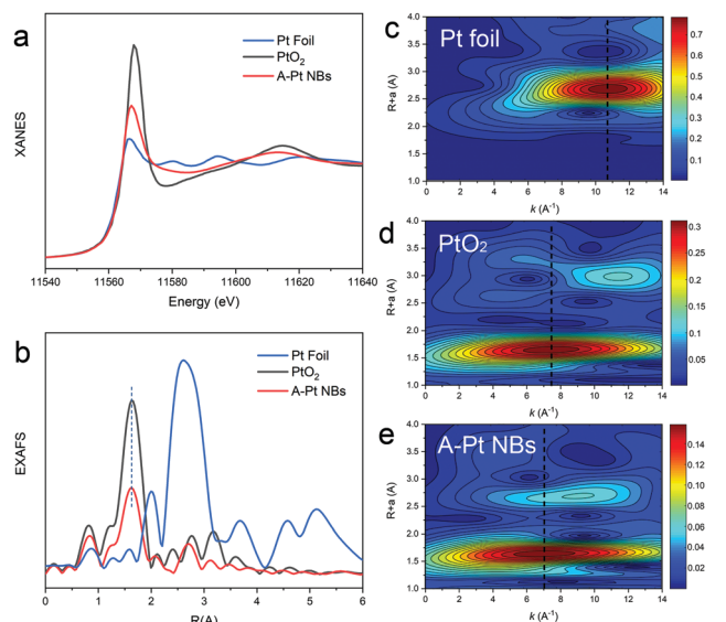
Fig. 3 X-ray absorption spectroscopic studies of the A-Pt NBs. (a) XANES spectra at the Pt \text{L}_3 -edge of the A-Pt NBs, \text{PtO}_2 , and Pt foil. (b) Fourier transform (FT) EXAFS spectrum of the A-Pt NBs compared with \text{PtO}_2 and Pt foil at the Pt \text{L}_3 -edge. (c–e) Wavelet transform (WT) EXAFS of the Pt foil (c), \text{PtO}_2 (d) and A-Pt NBs (e).
