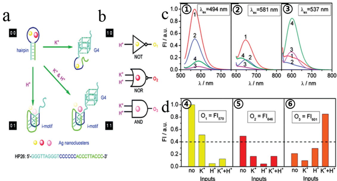
Fig. 2 (a) Schematic diagram of logic operations based on HP26-tuned fluorescent Ag NCs, with corresponding symbols of logic gates. K^+ and H^+ serve as two inputs to trigger the allotropy of HP26 and modulate the fluorescence output. (b) HP26-stabilized Ag NCs for multiple logic operations. (c, ①–③) Fluorescence emission spectra of Ag NCs at different excitation wavelength in 10 mM tris-Ac buffer (pH = 8.0) at four input modes: 1, no input; 2100 mM K^+ ; 3, H^+ (pH = 5.0); 4, K^+ and H^+ . (d, ④–⑥) Bar representations of the fluorescence intensity at 570 nm, 646 nm and 601 nm. The same threshold value (0.4) for output 1 or 0 is set at all fluorescence channels. Image reprinted from ref. 66 with permission. Copyright 2011 American Chemical Society.
