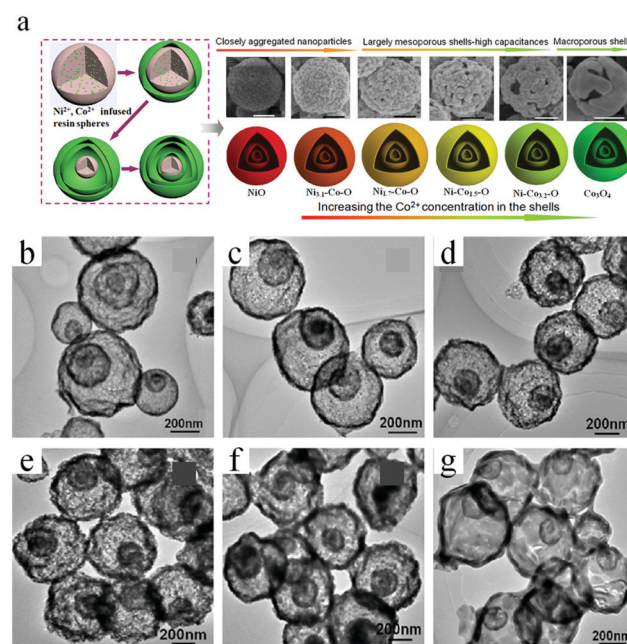
Fig. 15 (a) Schematic illustration of the preparation of triple-shelled \text{NiO} , \text{Co}_3\text{O}_4 , and their mixed oxide (Ni–Co–O) hollow spheres. (b–g) Typical TEM images of these samples. Reprinted from ref. 60 with kind permission.
