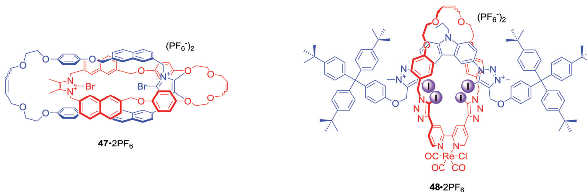
Fig. 23 First all-halogen examples of catenane and rotaxane.
