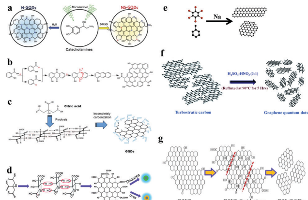
Fig. 2 Bottom-up synthesis of GQDs. (a) Preparation of N-doped GQDs and N,S-doped GQDs by a microwave-assisted method. (Reproduced with permission from ref. 34, copyright 2016 Wiley-VCH.) (b) Ultraviolet irradiation induces free-radical polymerization to prepare GQDs. (Reproduced with permission from ref. 35, copyright 2017 American Chemical Society.) (c) Preparation of GQDs with citric acid as a monomer. (Reproduced with permission from ref. 36, copyright 2012 Elsevier B.V.) (d) Preparation of N-doped GQDs and N,S-doped GQDs from graphene and urea or thiourea. (Reproduced with permission from ref. 37, copyright 2013 the Royal Society of Chemistry.) (e) Hybrids of GQDs and carbon nanoribbons were synthesized from toluene and hexabromobenzene. (Reproduced with permission from ref. 39, copyright 2015 American Chemical Society.) (f) GQDs cut from graphitized fine carbon powder obtained by decoupled roasting. (Reproduced with permission from ref. 40, copyright 2014 the Royal Society of Chemistry.) (g) GQDs obtained by ultrasonically assisted cutting of graphitized fine carbon powder. (Reproduced with permission from ref. 41, copyright 2016 American Chemical Society.)
