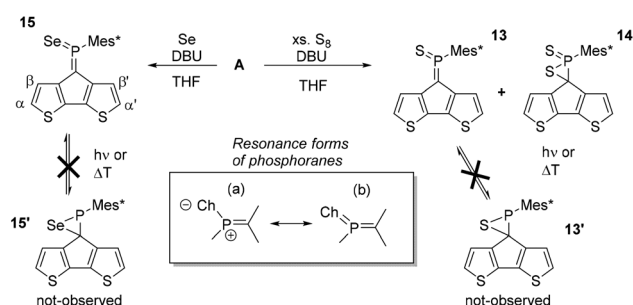
Scheme 3 Top: functionalisation of the CPDT phosphalkene using \text{S}_8 and \text{Se}_{\text{grey}} as oxidants. Thiaphosphorane 13 and selenophosphorane 15 could be isolated using column chromatography as ambiently stable compounds. Rearrangement of the thiaphosphorane into the thiaphosphirane was not observed under various conditions. Bottom: relevant resonance structures of the phosphoranes. The compound with a ^{31}\text{P} NMR resonance of -1.26 ppm was isolated by column chromatographic work-up. 2D NMR analysis indicates a \text{P–C}(\text{CPDT}) single bond, and the ^{31}\text{P} -NMR resonance agrees with the formation of 14 .
